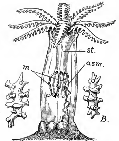
FIG. 3.—An expanded Alcyonarian zooid, showing the mouth surrounded by eight pinnate tentacles. st, Stomodaeum in the centre of the transparent body; m, mesenteries; asm, asulcar mesenteries; B, spicules, enlarged.
