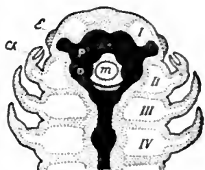
FIG. 5.—Diagram of the head and adjacent region of an Arachnid. Diprothomeric in the adult condition, though embryologically the appendages of somite II and the somite itself are, as here drawn, not actually in front of the mouth. E, Lateral eye. Ch, Chelicera. m, Mouth. P, Protocerebrum. D, Deutocerebrum. I, II, III, IV, Coelom of the first, second, third and fourth somites. (After Goodrich.)
