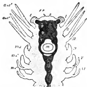
FIG. 6.—Diagram of the head of a Crustacean. Tri-prothomeric.
