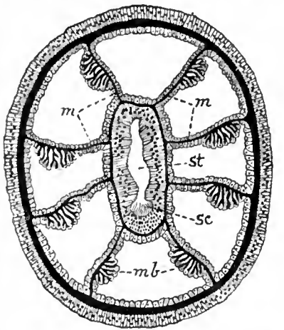
FIG. 4.—Transverse section of an Alcyonarian zooid. mm, Mesenteries; mb, muscle banners; sc, sulcus; st, stomodaeum.
