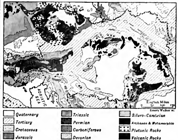
GEOLOGICAL MAP OF AUSTRIA-HUNGARY.
