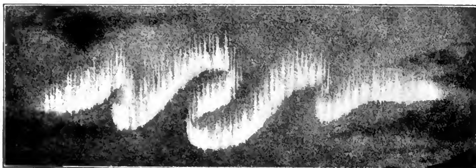
FIG. 3.—AURORAL BANDS.
