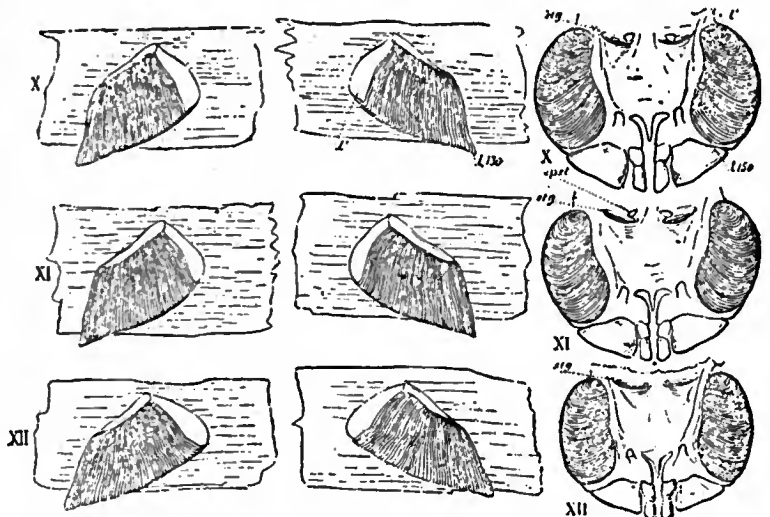
FIG. 15.—The remaining three pairs of mesosomatic appendages of Scorpio and Limulus . Letters as in fig. 14. h 130 indicates that there are 130 lamellae in the scorpion's lung-book, whilst h 150 indicates that 150 similar lamellae are counted in the gill of Limulus .
