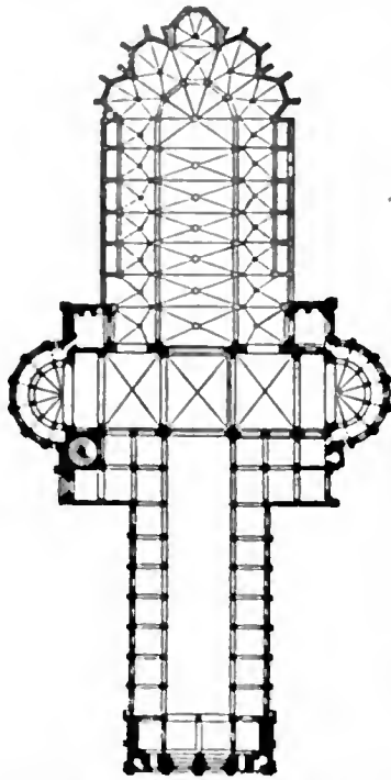
FIG. 49.—Plan of Cathedral at Tournai.
