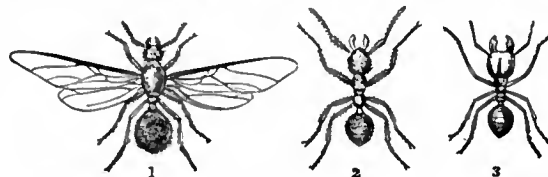
FIG. 2.—Leaf-cutting and Foraging Ants. 1, Atta cephalus ; 2, Eciton drepanophora ; 3, Eciton erratica .
