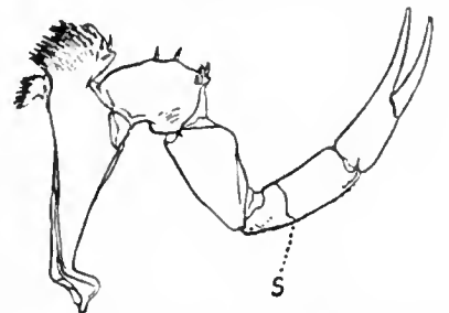
FIG. 11.—Third leg of Limulus polyphemus , showing the division of the fourth segment of the leg by a groove S into two, thus giving seven segments to the leg as in scorpion.
