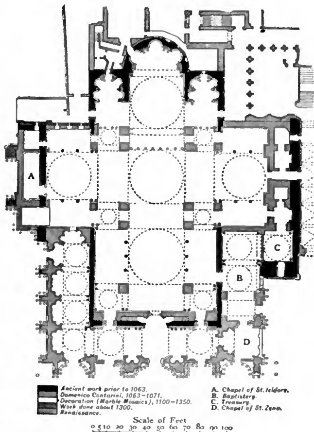
FIG. 37.—Plan of St Mark's, Venice.
