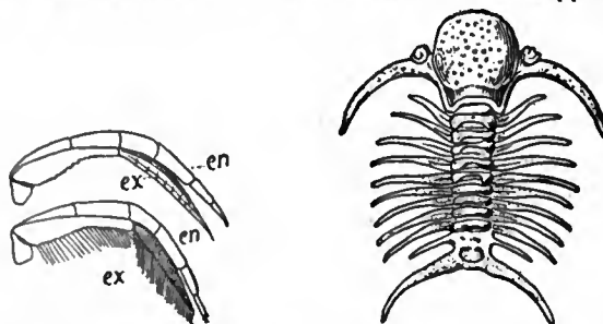
FIG. 36.— Triarthrus Becki , Green. Dorsal view of second thoracic leg with and without setae. en, Inner ramus; ex, Outer ramus.
