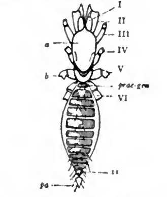
FIG. 58.— Schizomus crassicaudatus , a Tartarid Pedipalp. Dorsal view of a male with the appendages cut short.
