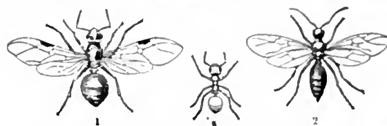
FIG. 1.—Wood Ant ( Formica rufa ). 1, Queen; 2, male; 3, worker.
