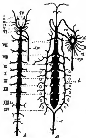
FIG. 29.—Diagram of the arterial system of A, Scorpio , and B, Limulus . The Roman numerals indicate the body somites and the two figures are adjusted for comparison. ce, Cerebral arteries; sp, supra-spinal or medullary artery; c, caudal artery; l, lateral anastomotic artery of Limulus . The figure B also shows the peculiar neural investiture formed by the cerebral arteries in Limulus and the derivation from this of the arteries to the limbs, III, IV, VI, whereas in Scorpio the latter have a separate origin from the anterior aorta.
