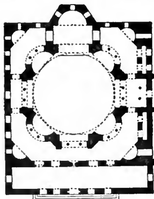
FIG. 27.—Plan of SS. Sergius and Bacchus.
