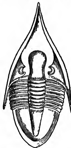
FIG. 39.— Megalaspis extenuatus . One of the Asaphidae allied to Illaeus , from the Ordovician of East Gothland, Sweden.
