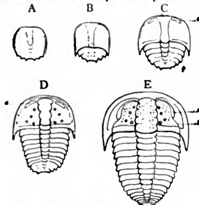
FIG. 41.—Five stages in the development of the trilobite Sao hirsuta .
