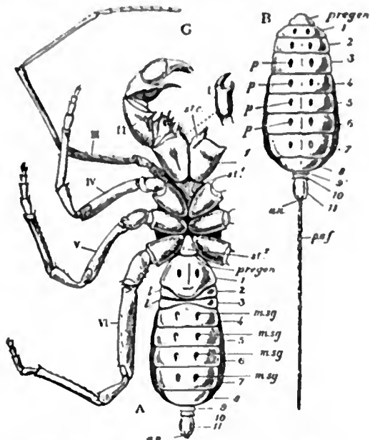
FIG. 54.— Thelyphonus , one of the Pedipalpi.
