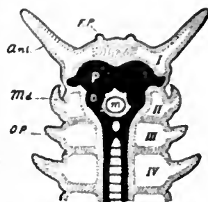
FIG. 4.—Diagram of the head and adjacent region of Peripatus . Monoprothomeric.
