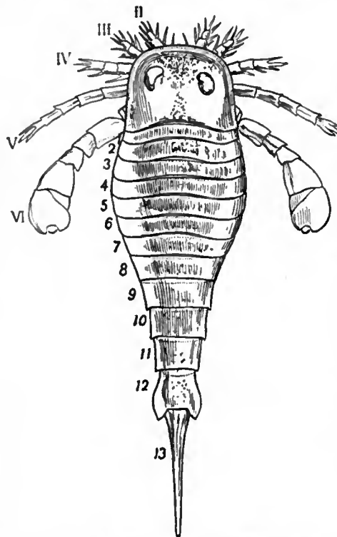
FIG. 46.— Eurypterus Fischeri , Eichwald. Silurian of Rootzikil. Restoration after Schmidt, half the size of nature. The dorsal aspect is presented showing the prosomatic shield with paired compound eyes and the prosomatic appendages II. to VI. The small first pair of appendages is concealed from view by the carapace. 1 to 12 are the somites of the opisthosoma; 13, the post-anal spine.
