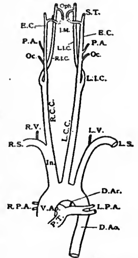
FIG. 4.—Diagram of the Human Aorta and its branches. S.T., Superficial Temporal Artery.
