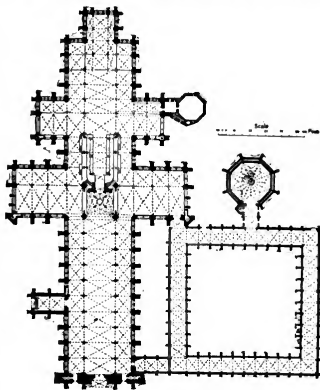
FIG. 43.—Plan of Salisbury Cathedral.
