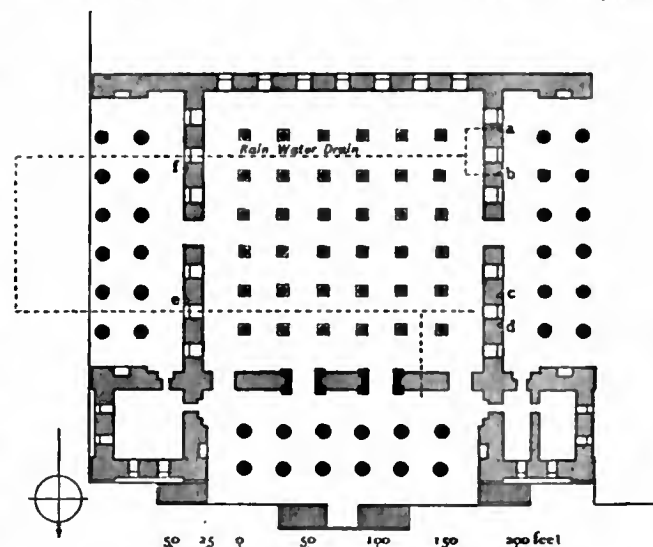
FIG. 13.—Plan of the Hall of Xerxes.
