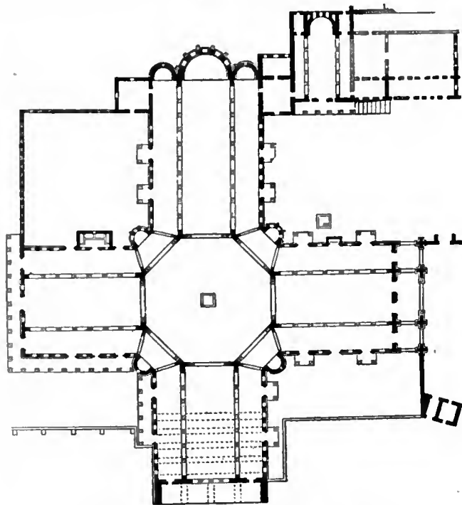
FIG. 34.—Plan of Church of Kalat-Seman.
