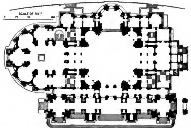
FIG. 112.—Plan of Cathedral at Berlin.
