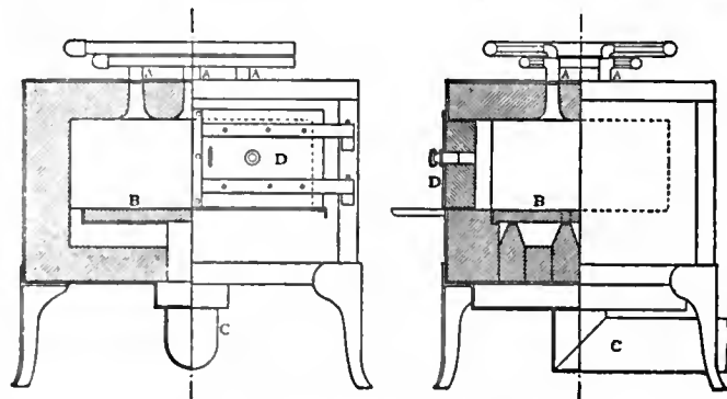
FIG. 2.—Reverberatory Furnace.
