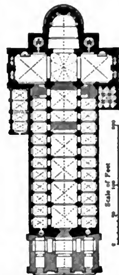
FIG. 47.—Plan of Cathedral at Spire.
