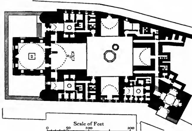
FIG. 57.—Plan of the Mosque of the Sultan Hasan.
