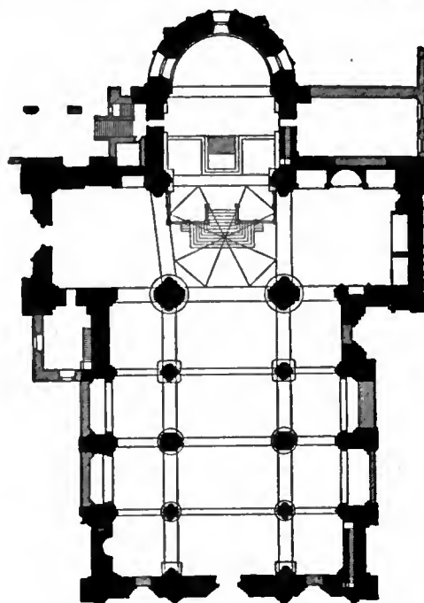
FIG. 36.—Plan of San Michele, Pavia.
